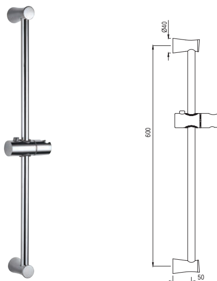
SHA-1197N Sliding Rail \phi 19mm & 600mm Long Round Shape with Hand Shower Holder
