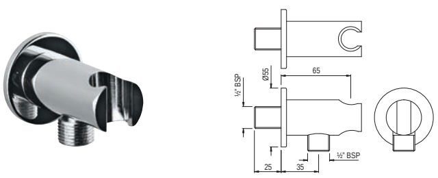
SHA-566R Wall Outlet with Shower Hook in Round Shape
