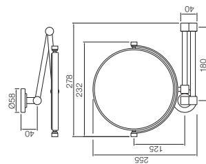
ACN-1193N Double Arm Wall Mounted Reversible Plain / Magnifying (X3) Pivotal Mirror
