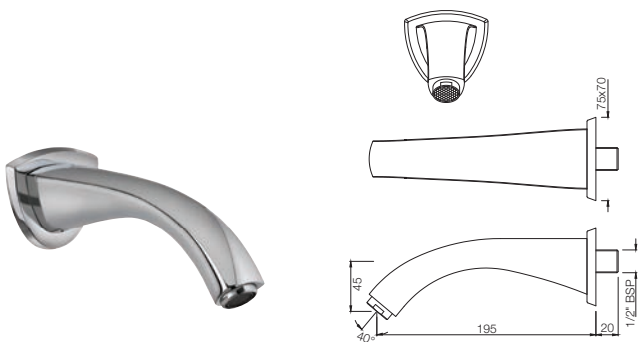
SPJ-87429 Bath Tub Spout with Wall Flange
