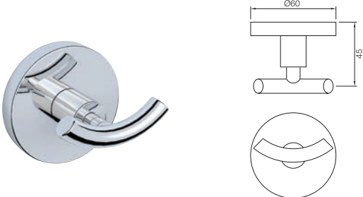
ACN-1161N Double Coat Hook
