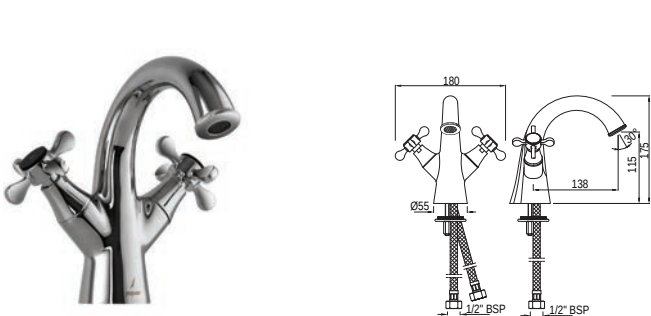
QQP-7167BPM Central Hole Basin Mixer without Popup Waste System with 450mm Long Braided Hoses
