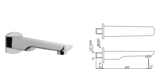
SPJ-35429PM Bathtub Spout with Wall Flange
