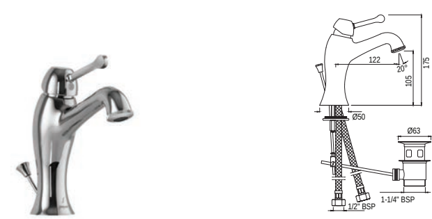
QQP-7051BPM Single Lever Basin Mixer with Popup Waste with 450mm Long Braided Hoses
