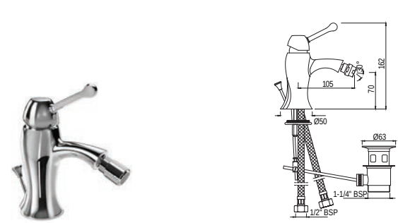
QQP-7213BPM Single Lever 1-Hole Bidet Mixer with Popup Waste System with 375mm Long Braided Hoses
