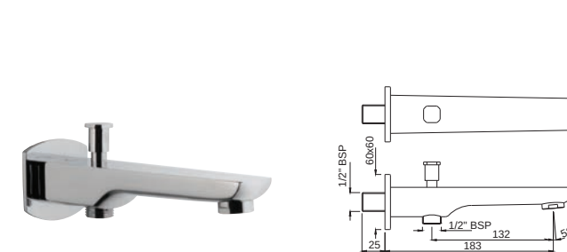
SPJ-35463PM Bathtub Spout with Button Attachment for Hand Shower with Wall Flange
