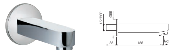
SPJ-29429 Bathtub Spout with Wall Flange
