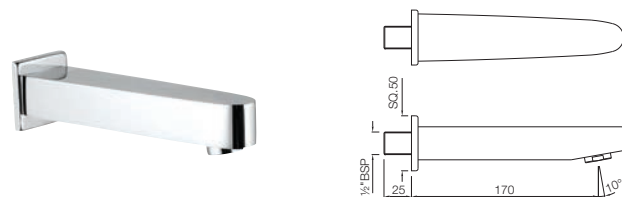
SPJ-81429 Bathtub Spout with Wall Flange
