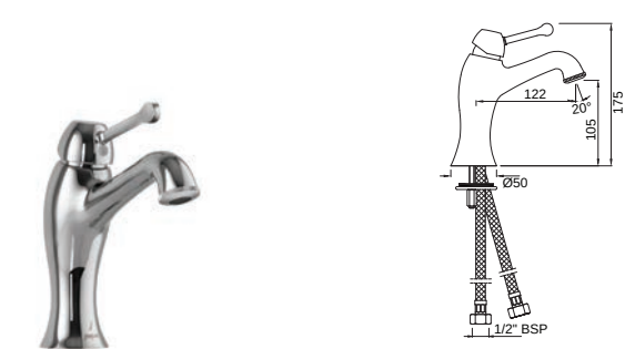
QQP-7001BPM Single Lever Basin Mixer without Popup Waste with 450mm Long Braided Hoses
