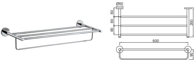
ACN-1181S Towel Rack 600mm Long with Lower Hangers, Stainless Steel
