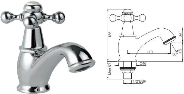
QQT-7011 Pillar Cock
