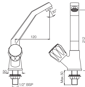
CON-359KN Sink Cock with Raised 'J' Shaped Swinging Spout (Table Mounted Model)
