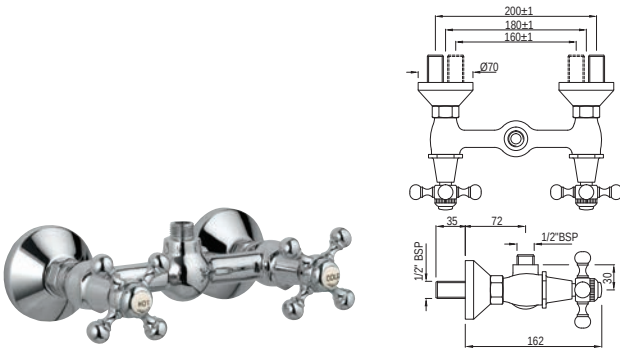
QQT-7209 Shower Mixer for Shower Cubicles (Wall Mounted) with Connecting Legs & Flanges
