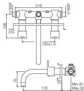
FUS-29433 Two Concealed Stop Cocks with Basin Spout (Composite One Piece Body)
