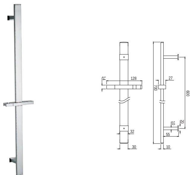
SHA-1183 Sliding Rail 700X30X10mm Flat Shape with Hand Shower Holder
