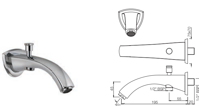
SPJ-87463 Bath Tub Spout with Button attachment for Hand Shower with Wall Flange
