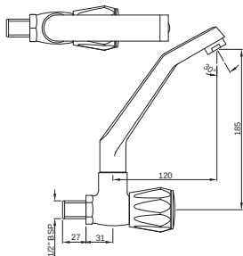
CON-357KN Sink Cock with Raised 'J' Shaped Swinging Spout (Wall Mounted Model)
