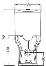
BACK VIEW
