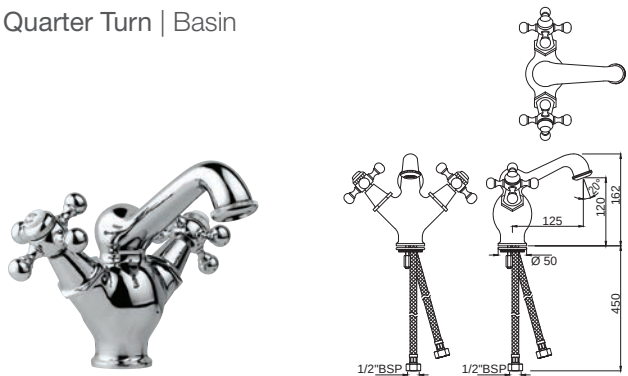
QQT-7167B Central Hole Basin Mixer with Regular Spout without Popup Waste System with 450mm Long Braided Hoses
