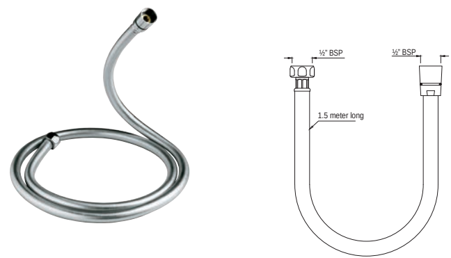
SHA-571 Easy Flex Tube in Chrome Finish 1.5m Long with Nuts
