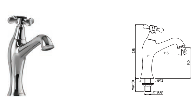
QQP-7011PM Pillar Cock
