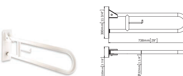
WAC-WHT-BG0800 Grab Bar Vertical Swing, White
