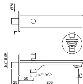
SPJ-CHR-91463 Bathtub spout with button attachment for hand shower with wall flange
