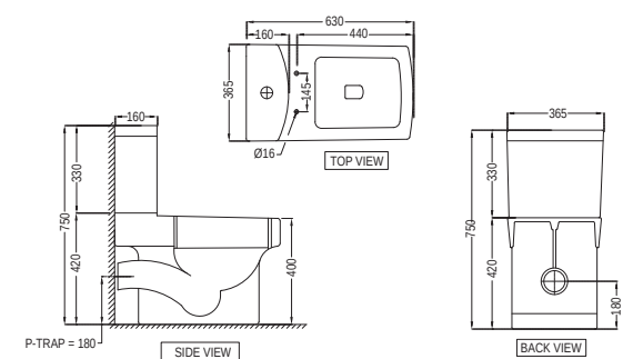
Floor mounted coupled WC FNS-WHT-40751P180UFSM Bowl for Coupled WC with UF soft close slim seat cover, Hinges, Fixing Accessories and Accessories Set, Size: 365x630x750 mm, P Trap-180mm FNS-WHT-40201 Cistern with cistern fittings for- 40751P180UFSM & 40751S220UFSM
