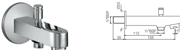
SPJ-29463 Bathtub Spout with Button Attachment for Hand Shower with Wall Flange
