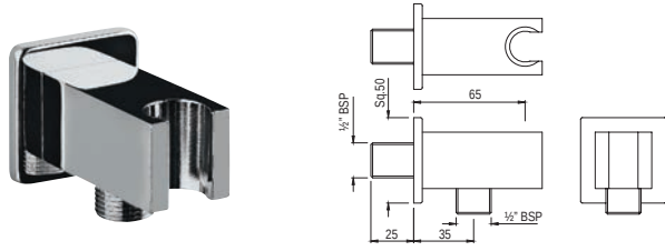
SHA-566S Wall Outlet with Shower Hook in Square Shape
