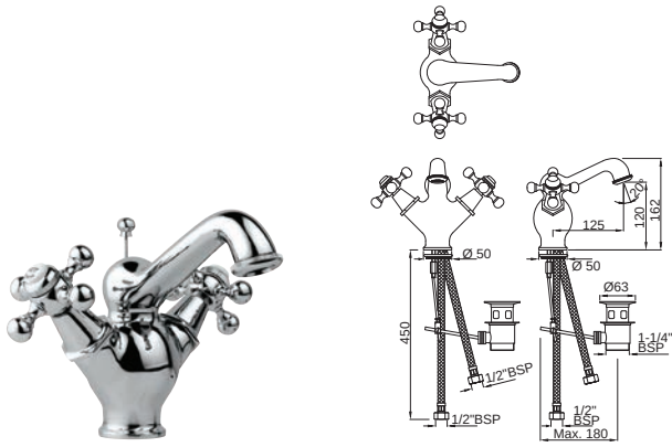
QQT-7169B Central Hole Basin Mixer with Regular Spout with Popup Waste System with 450mm Long Braided Hoses
