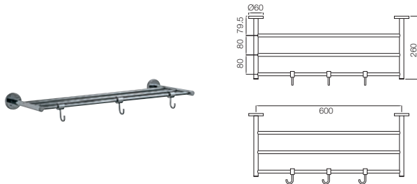
ACN-1181FHS Towel Rack 600mm Long without Lower Hangers but with 3 hooks, Stainless Steel
