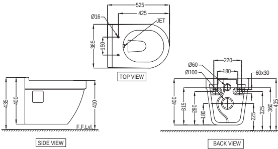
SLS-WHT-6951JPPSM Wall Hung WC with In built Jet, PP Soft Close Slim Seat, Hinges, Accessories Set, Size:365x525x400 mm
