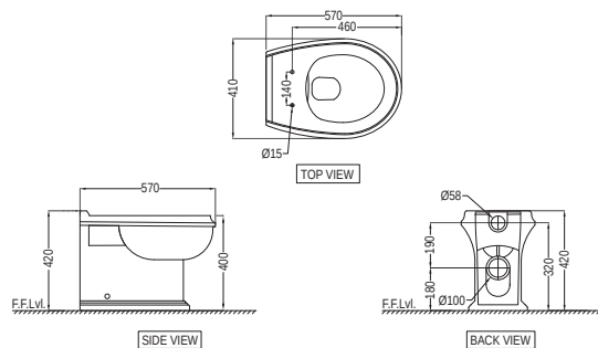
QPS-WHT-7955P180UFPM Rimless Back To Wall WC With UF Soft Close Seat Cover, Hinges, Fixing Accessories And Accessories Set, Size: 410x570x420 mm, P Trap- 180 mm
