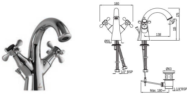
QQP-7169BPM Central Hole Basin Mixer with Popup Waste System with 450mm Long Braided Hoses
