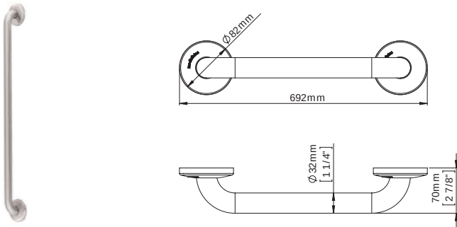
WAC-SAP-BR0600CS Grab Bar 692 mm Long, Satin
