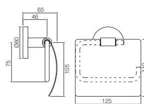
ACN-1153S Toilet Roll Holder with Stainless Steel Flap
