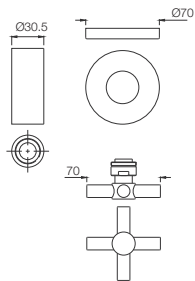
SOL-6083K Exposed Part Kit of Concealed Stop Cock & Flush Cock with Fitting Sleeve, Operating Lever & Adjustable Wall Flange with Seal (compatible with ALD-083, ALD-089 & ALD-081)
