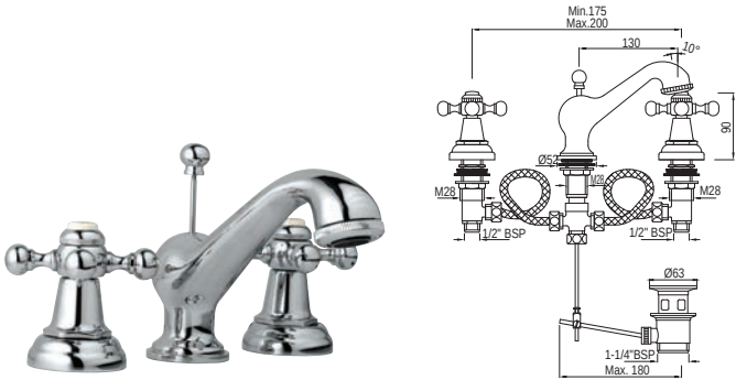
QQT-7191 3-Hole Basin Mixer with Popup Waste System
