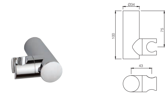
SHA-555 Premium Wall Bracket for Hand Shower, ø35mm & 100mm Long Round Shape
