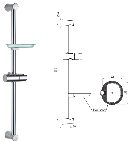
SHA-1187N Sliding Rail \phi 19mm & 600mm Long Round Shape with Hand Shower Holder & Soap Dish
