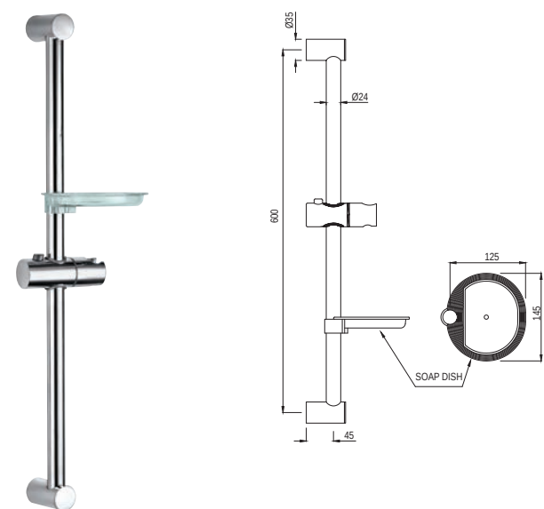
SHA-1189N Sliding Rail \phi 24mm & 600mm Long Round Shape with Hand Shower Holder & Soap Dish
