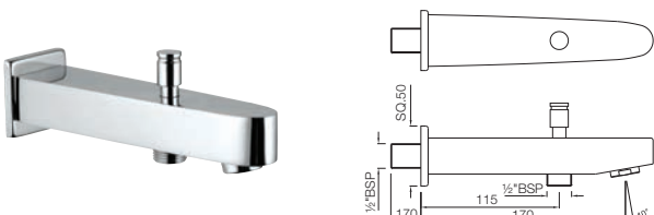
SPJ-81463 Bathtub Spout with Button Attachment for Hand Shower with Wall Flange
