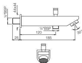
SPJ-37463 Bathtub Spout with Button Attachment for Hand Shower with Wall Flange
