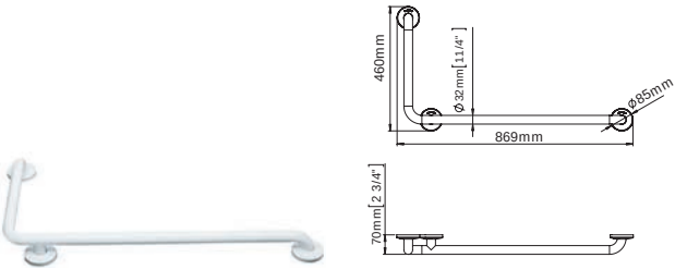
WAC-WHT-BAI090 Grab Bar Left 90° Angle, White
